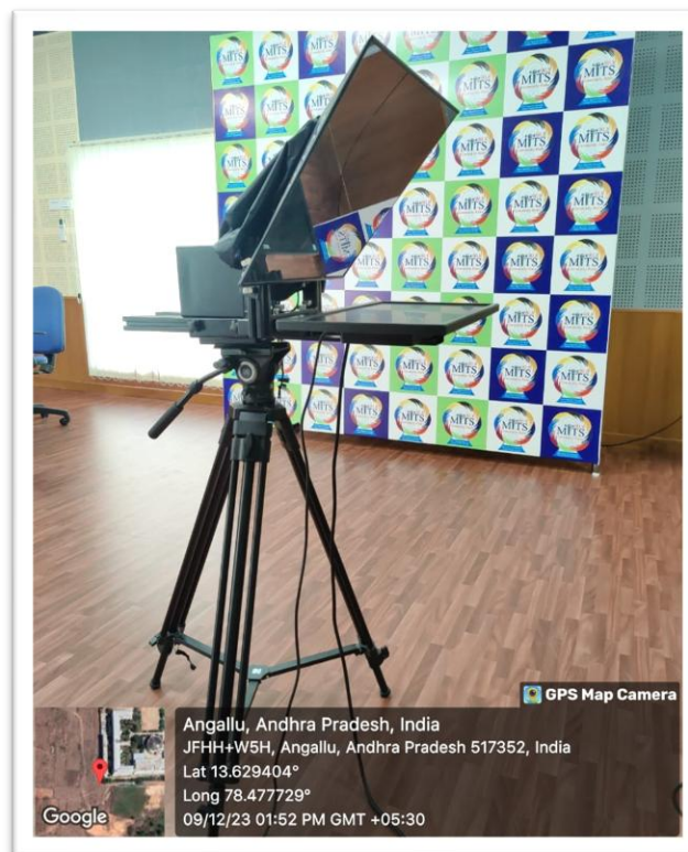
Figure 4. Teleprompter with remote and software
